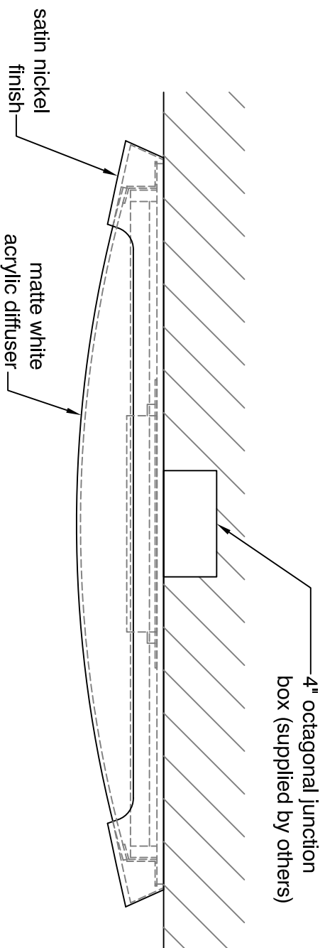
TOP VIEW
