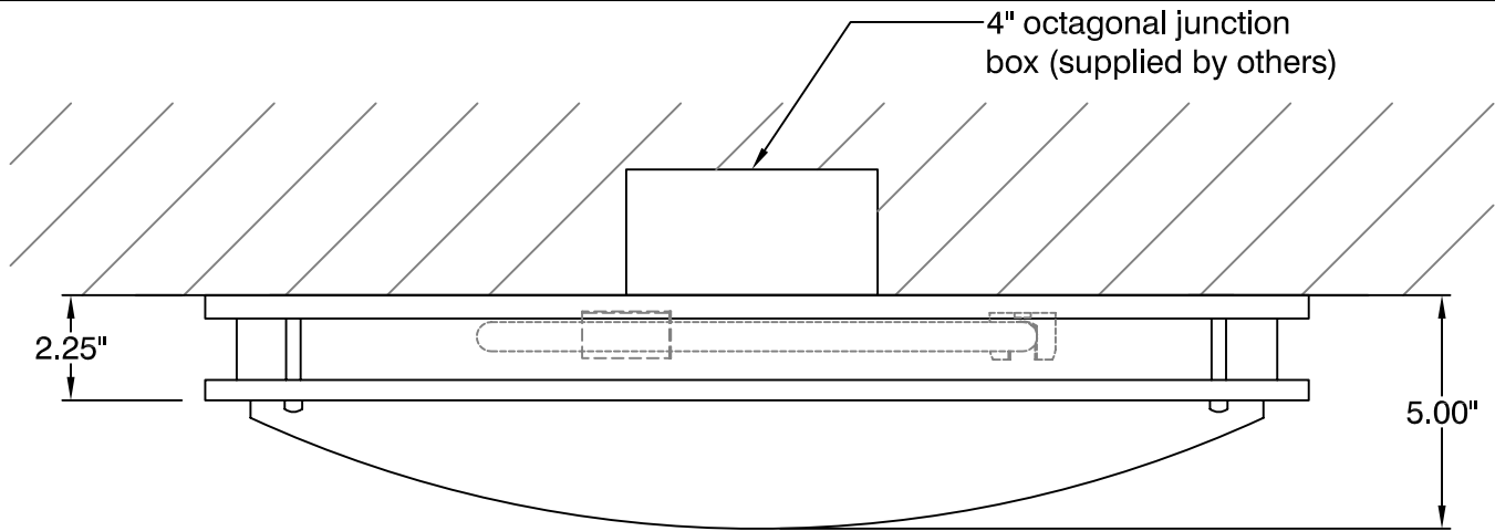
SIDE VIEW
