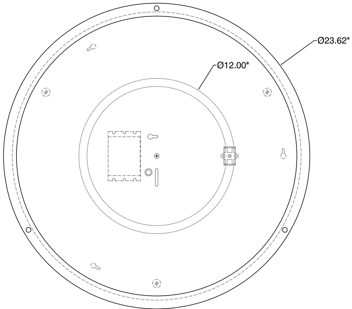
BOTTOM VIEW
