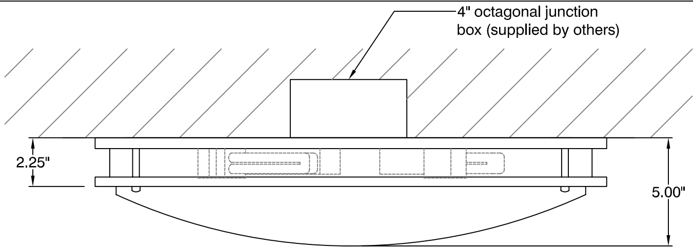
SIDE VIEW
