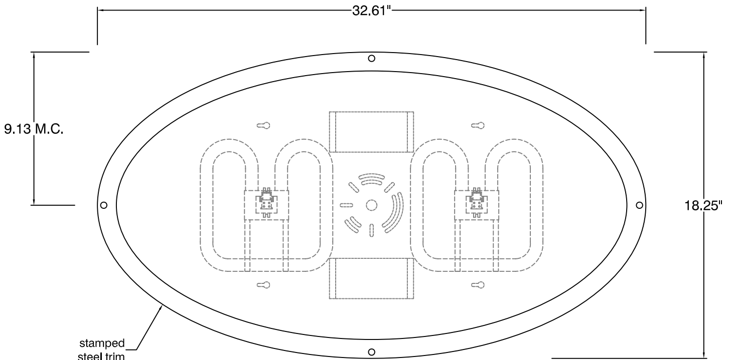
BOTTOM VIEW
