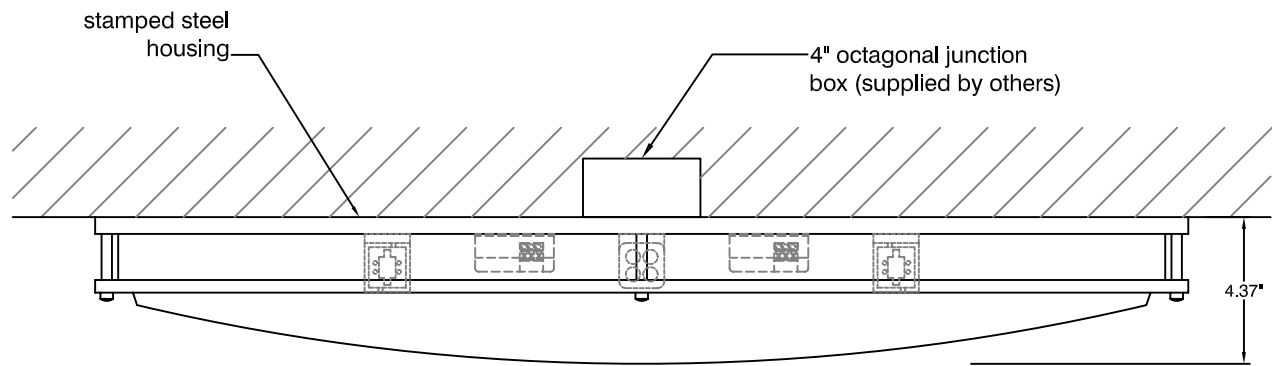
SIDE VIEW
