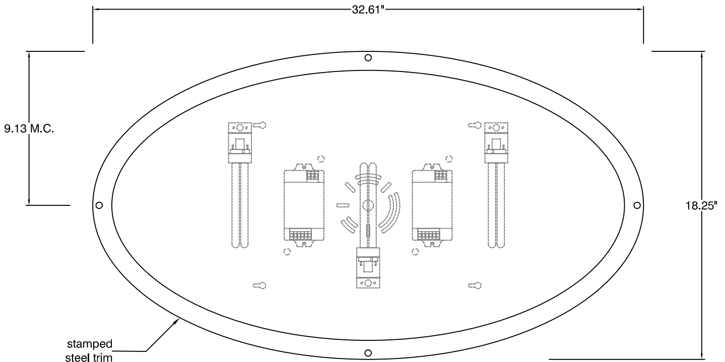
BOTTOM VIEW
