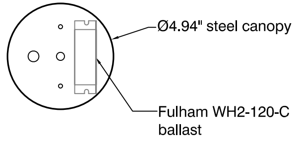
TOP VIEW (canopy)
