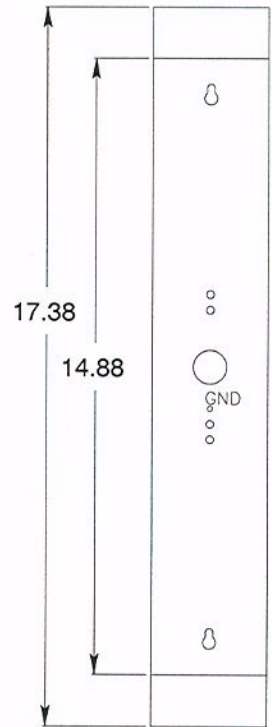
MOUNTING PLATE
