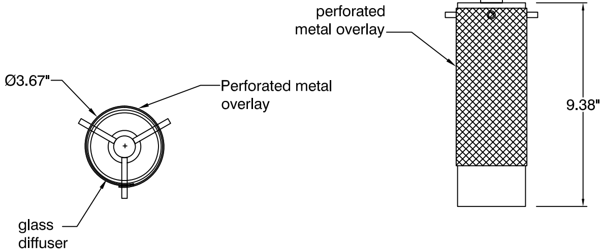
TOP VIEW (diffuser)
