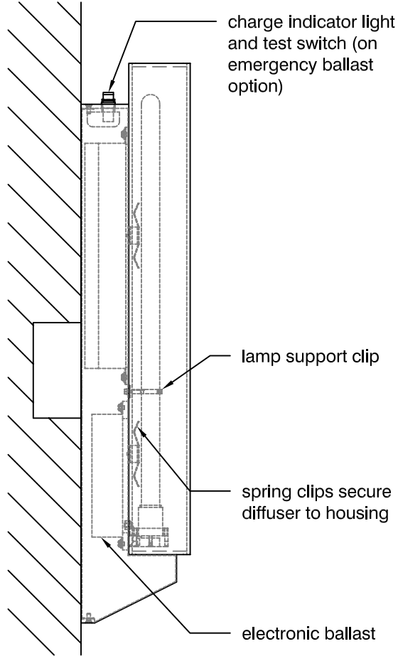
SIDE VIEW
